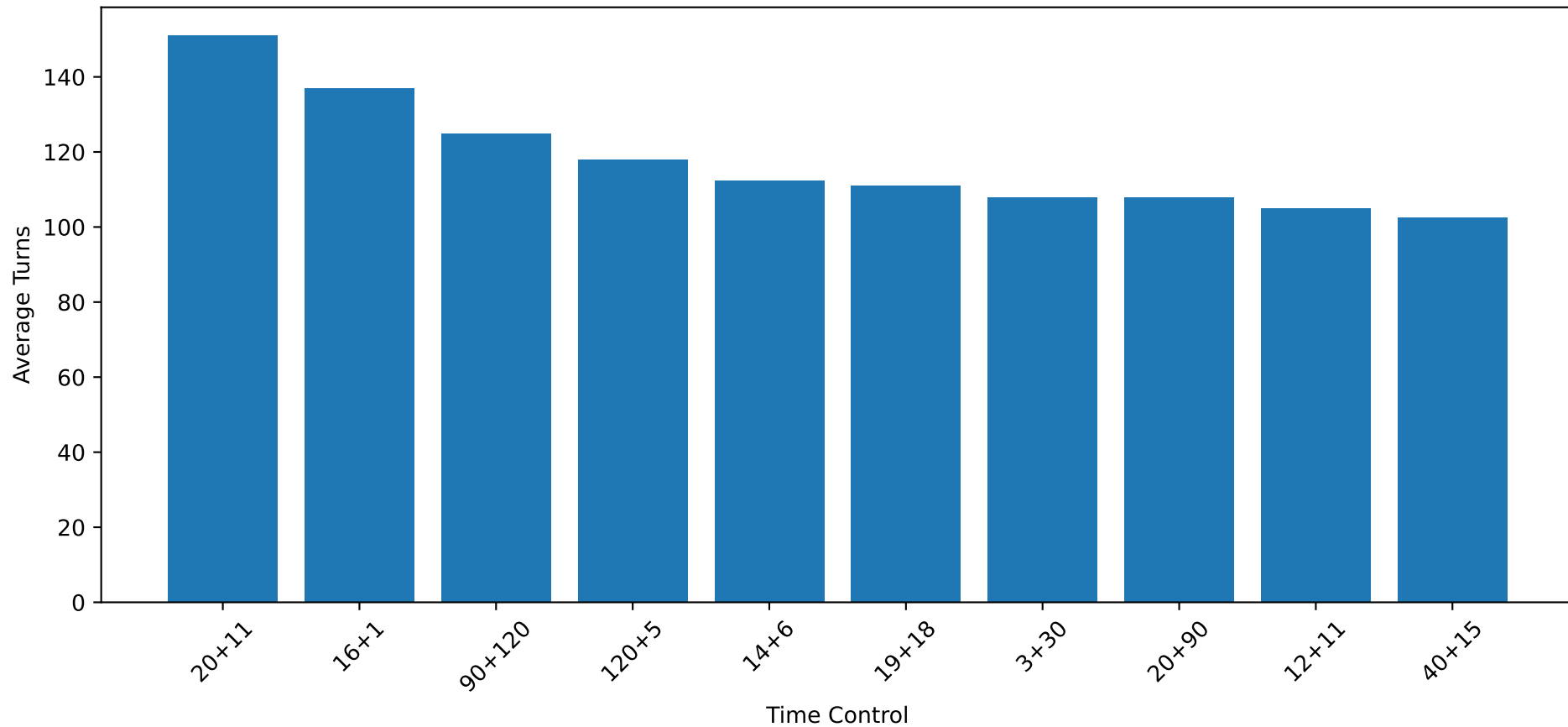
Time Control vs Game Duration
